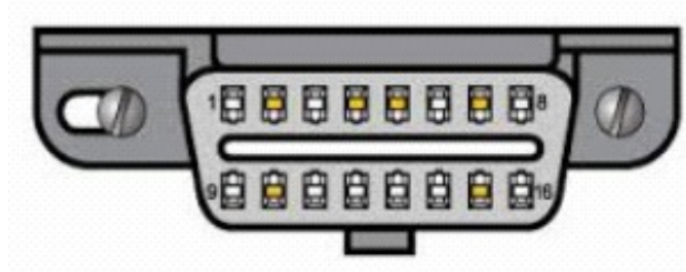
OBD-II service connector
